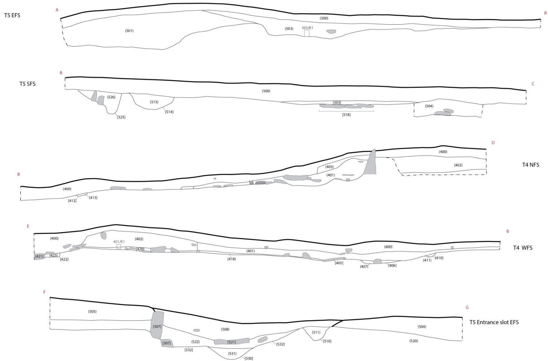
Figure 14: Trenches 4 & 5 sections
